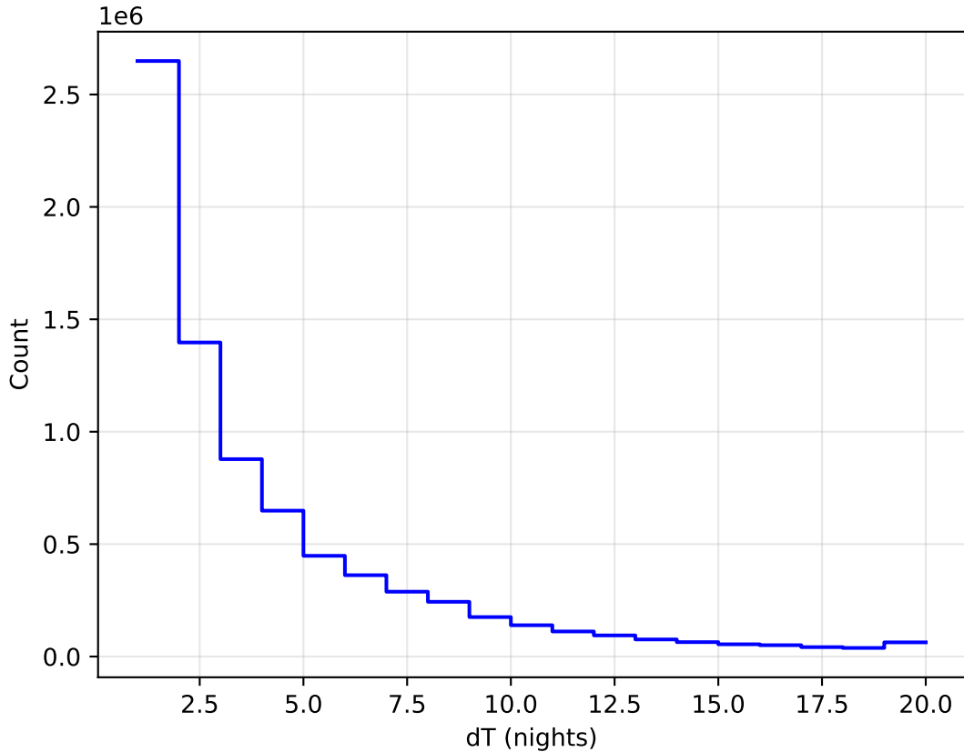
ddf_acor_sf10_lsf40_lsr20_v3.4_10yrs WFD all bands: DeltaNight Histogram
