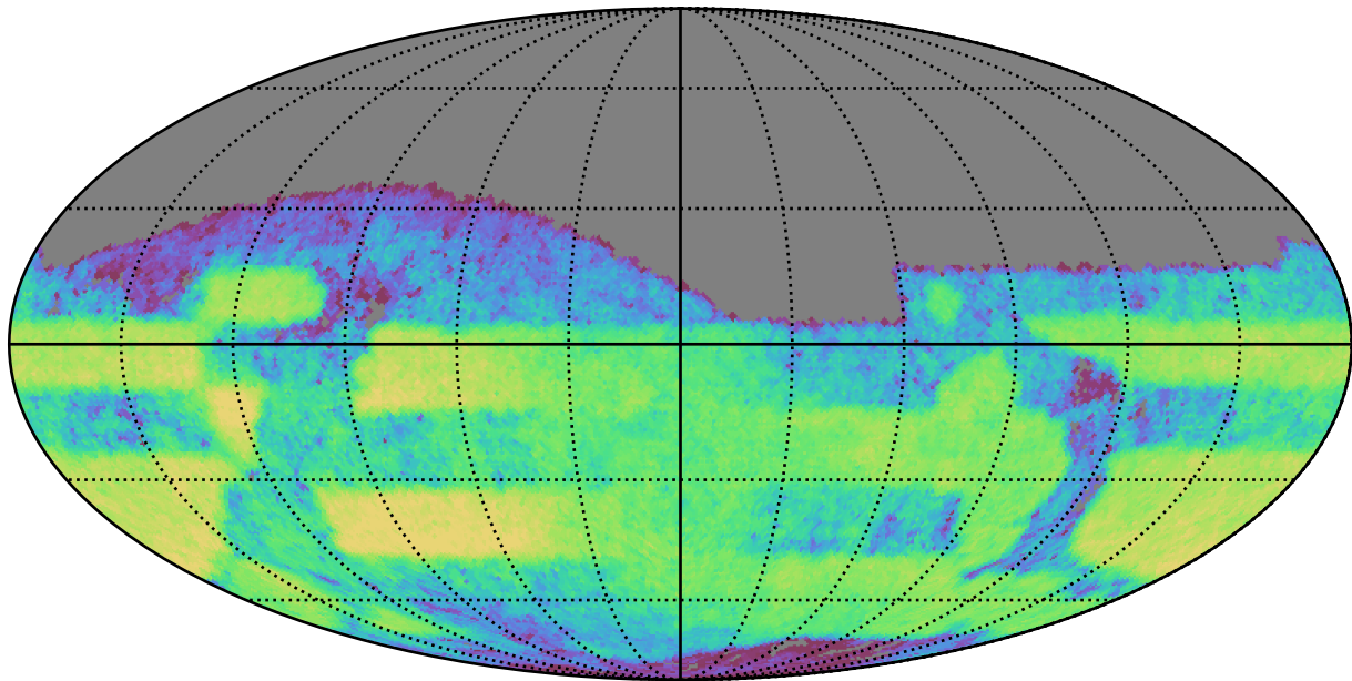
ddf_acor_sf10_lsf40_lsr20_v3.4_10yrs Yr 3-4 r band: CoaddM5
