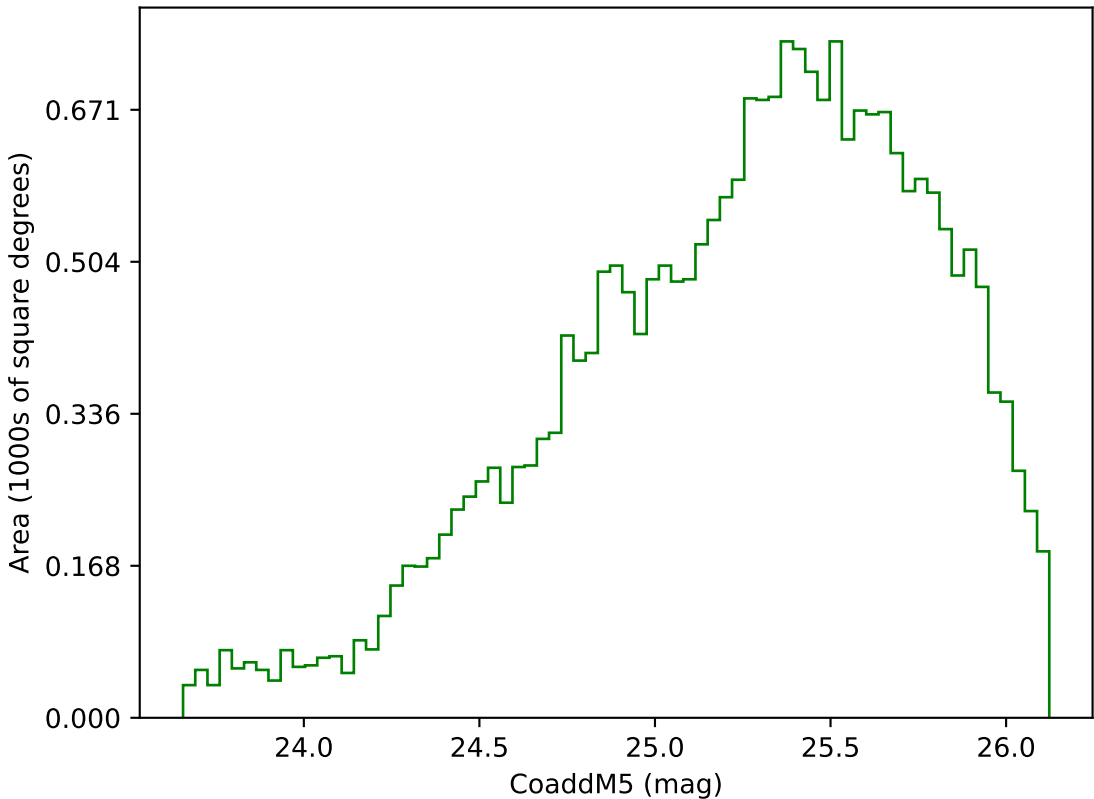
ddf_acor_sf10_lsf40_lsr20_v3.4_10yrs Yr 3-4 g band: CoaddM5
