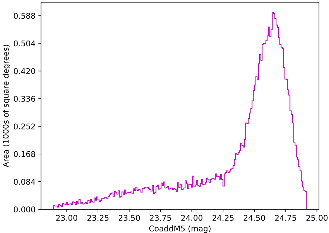
ddf_acor_sf10_lsf40_lsr20_v3.4_10yrs Yr 1 z band: CoaddM5
