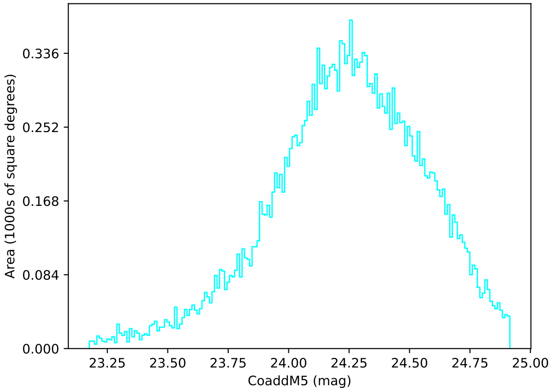
ddf_acor_sf10_lsf40_lsr20_v3.4_10yrs Yr 1 u band: CoaddM5
