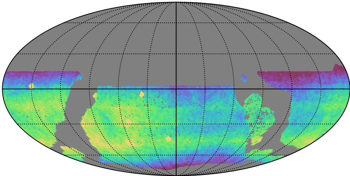
ddf_acor_sf10_lsf40_lsr20_v3.4_10yrs WFD r band: CoaddM5
