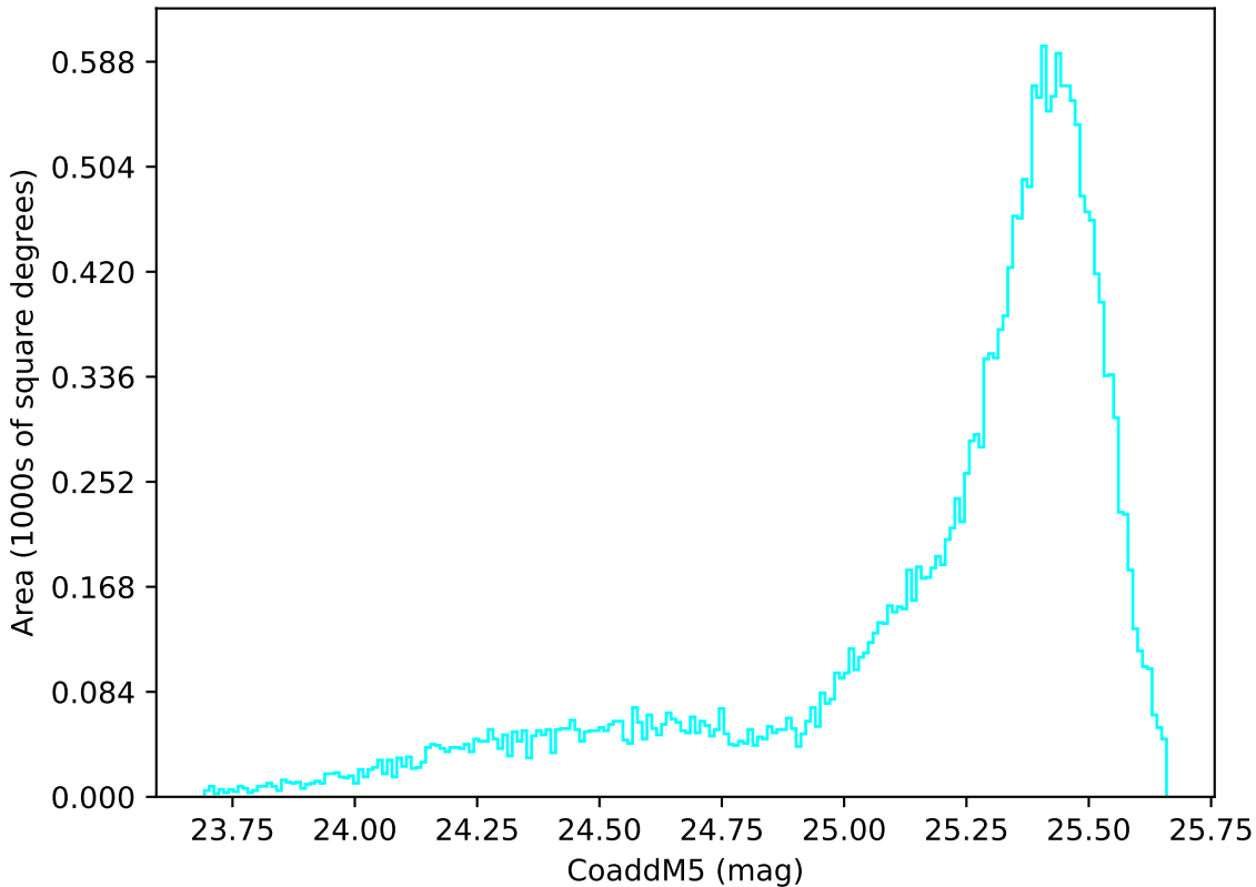
ddf_acor_sf10_lsf40_lsr20_v3.4_10yrs All sky u band: CoaddM5
