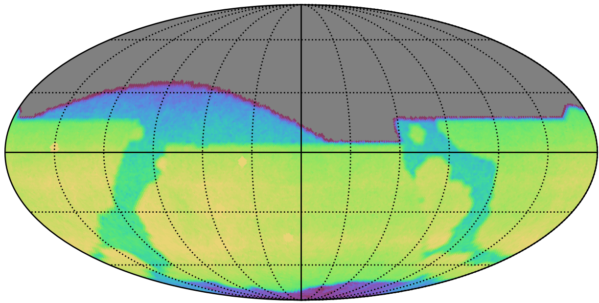
ddf_acor_sf10_lsf40_lsr20_v3.4_10yrs All sky r band: CoaddM5
