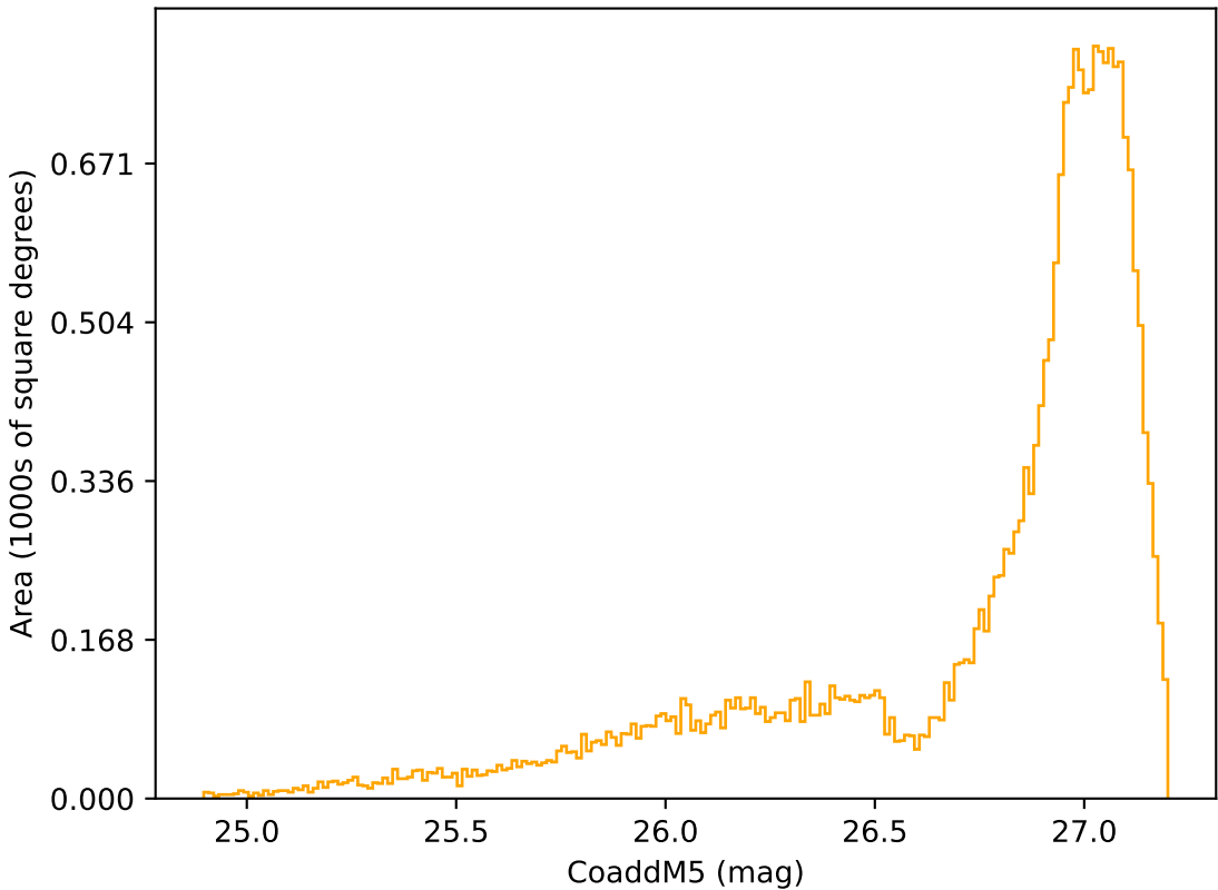
ddf_acor_sf10_lsf40_lsr20_v3.4_10yrs All sky r band: CoaddM5
