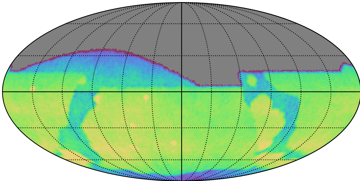
ddf_acor_sf10_lsf40_lsr20_v3.4_10yrs All sky g band: CoaddM5
