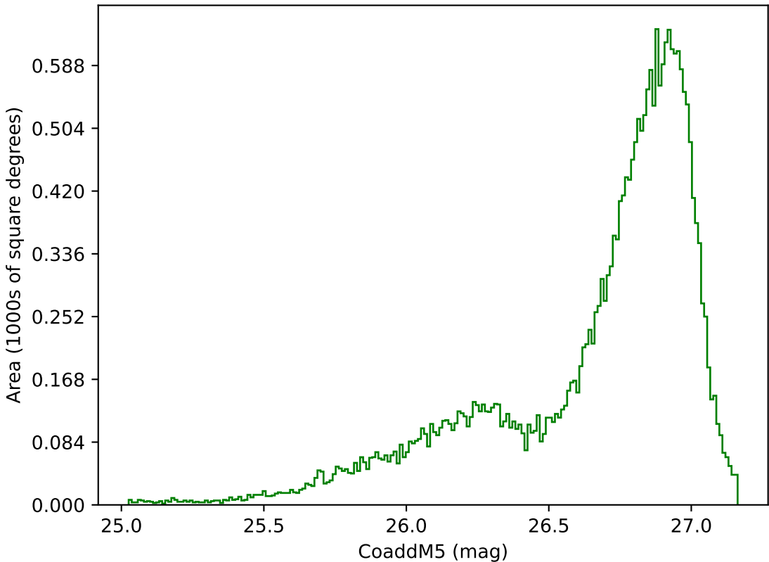
ddf_acor_sf10_lsf40_lsr20_v3.4_10yrs All sky g band: CoaddM5
