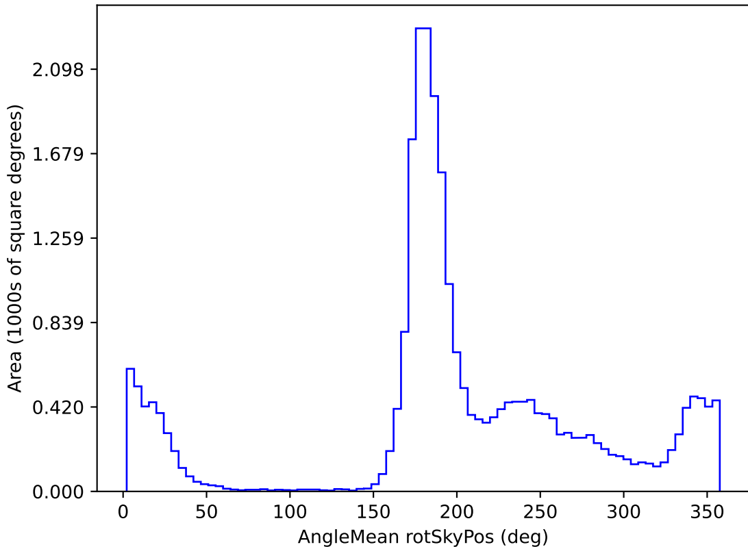
ddf_acor_sf10_lsf40_lsr20_v3.4_10yrs All sky r band: AngleMean rotSkyPos
