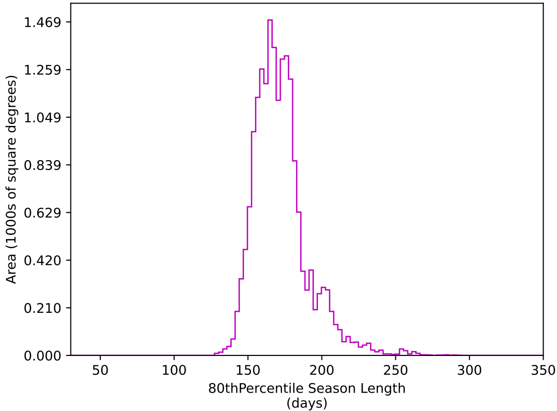
ddf_acor_sf10_lsf40_lsr20_v3.4_10yrs WFD z band: 80thPercentile Season Length
