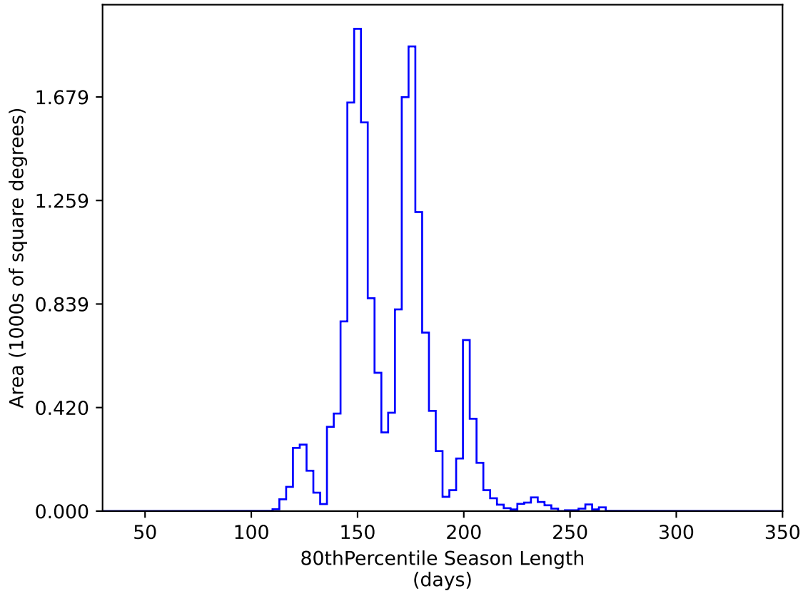
ddf_acor_sf10_lsf40_lsr20_v3.4_10yrs WFD y band: 80thPercentile Season Length
