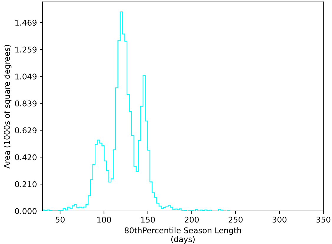
ddf_acor_sf10_lsf40_lsr20_v3.4_10yrs WFD u band: 80thPercentile Season Length
