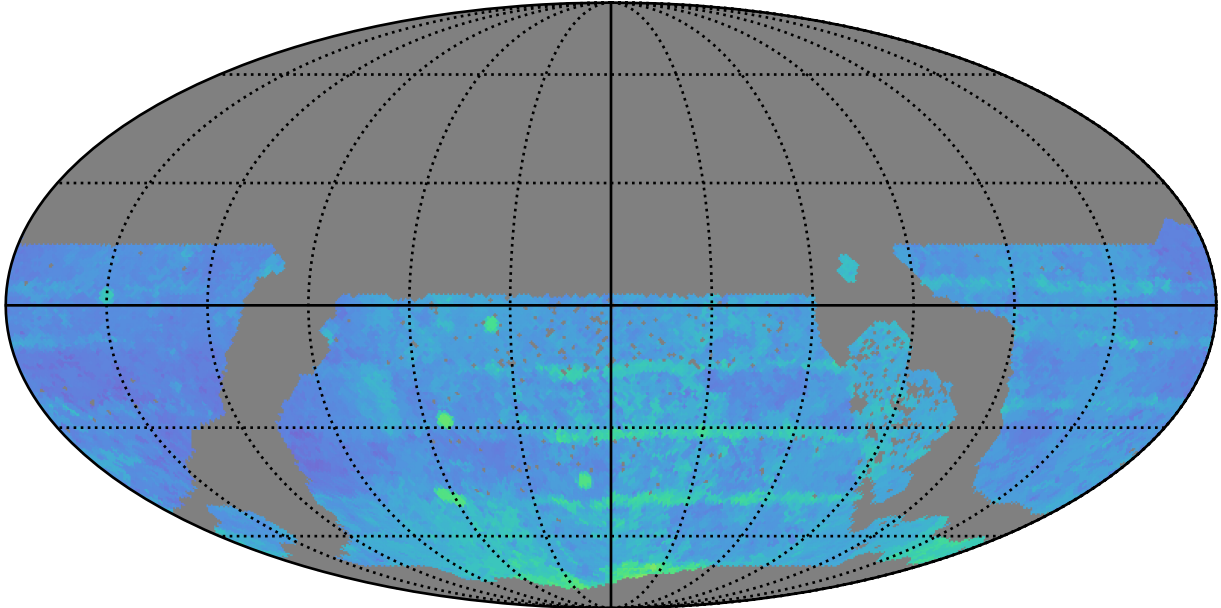
ddf_acor_sf10_lsf40_lsr20_v3.4_10yrs WFD r band: 80thPercentile Season Length
