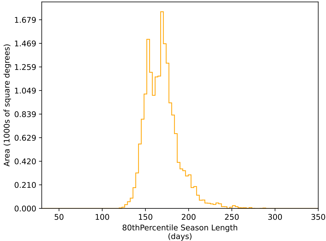
ddf_acor_sf10_lsf40_lsr20_v3.4_10yrs WFD r band: 80thPercentile Season Length
