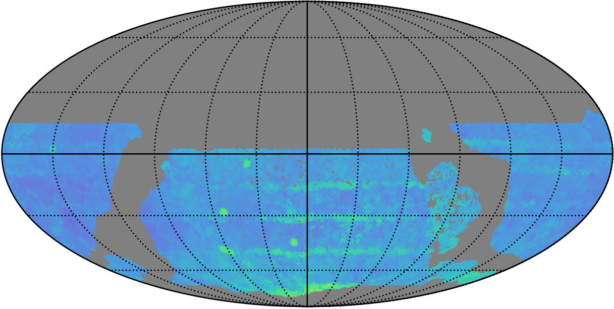
ddf_acor_sf10_lsf40_lsr20_v3.4_10yrs WFD i band: 80thPercentile Season Length
