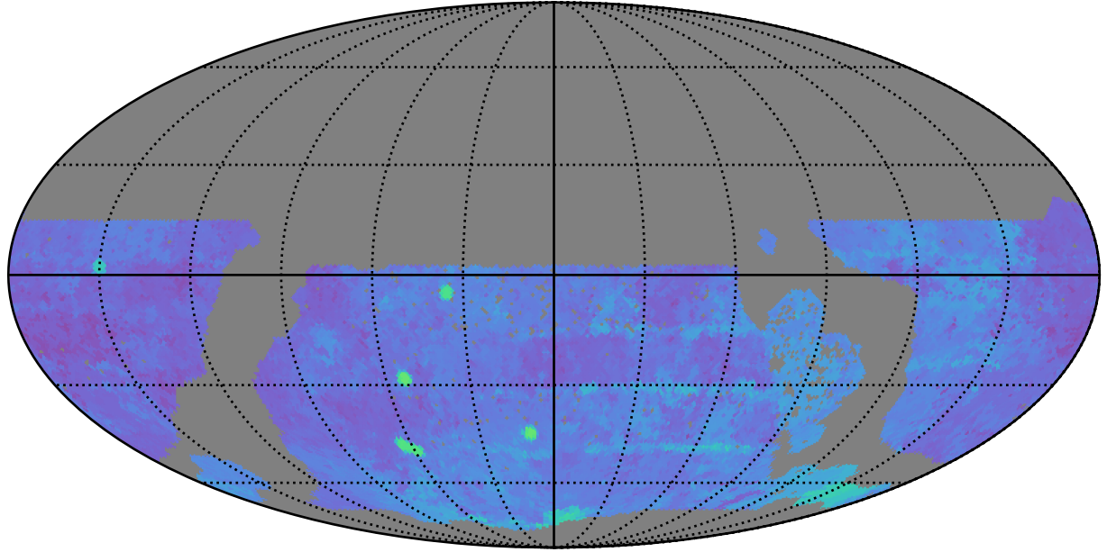
ddf_acor_sf10_lsf40_lsr20_v3.4_10yrs WFD g band: 80thPercentile Season Length
