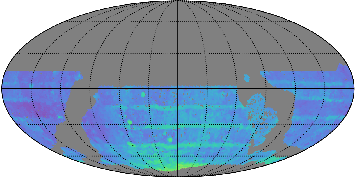
ddf_acor_sf10_lsf40_lsr20_v3.4_10yrs WFD all bands: 80thPercentile Season Length
