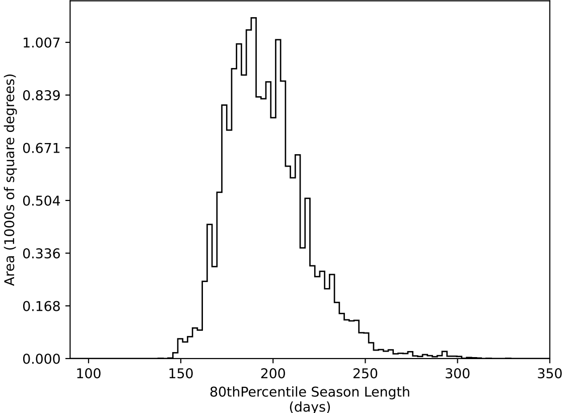
ddf_acor_sf10_lsf40_lsr20_v3.4_10yrs WFD all bands: 80thPercentile Season Length
