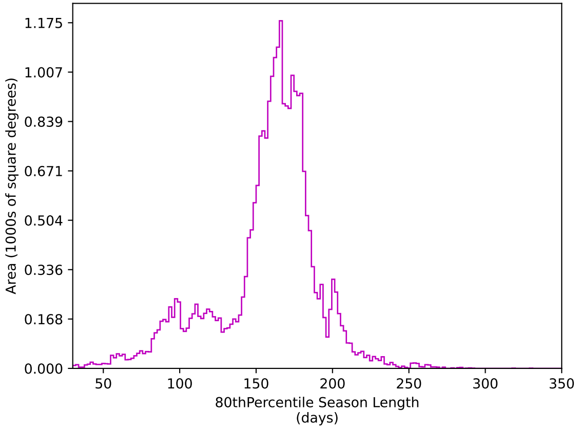
ddf_acor_sf10_lsf40_lsr20_v3.4_10yrs All sky z band: 80thPercentile Season Length
