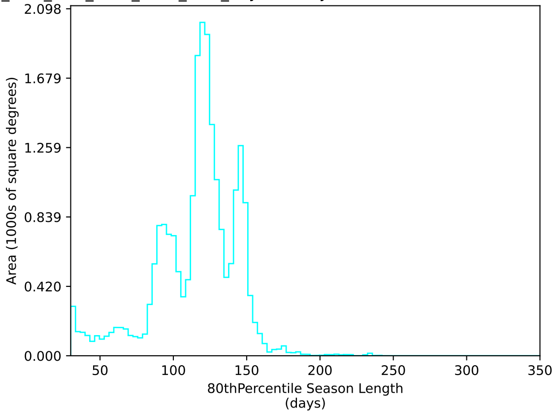
ddf_acor_sf10_ls40_lsr20_v3.4_10yrs All sky u band: 80thPercentile Season Length
