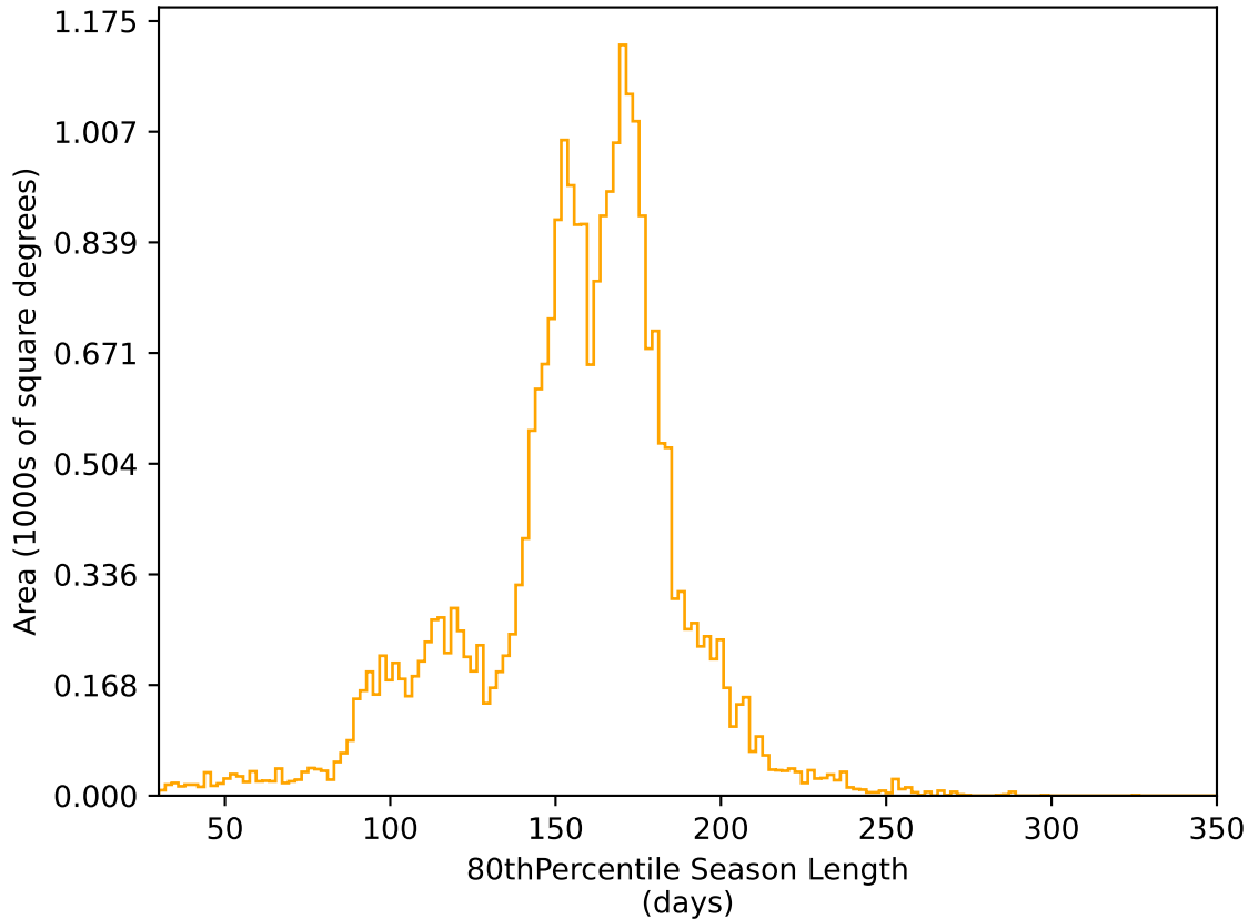
ddf_acor_sf10_lsf40_lsr20_v3.4_10yrs All sky r band: 80thPercentile Season Length
