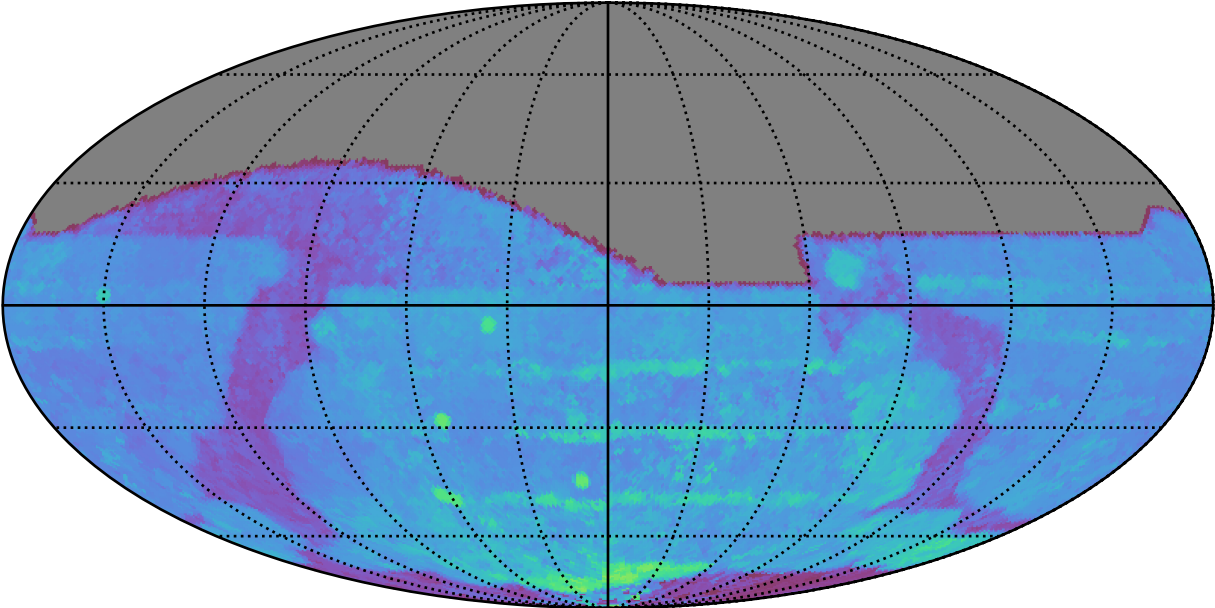
ddf_acor_sf10_lsf40_lsr20_v3.4_10yrs All sky i band: 80thPercentile Season Length
