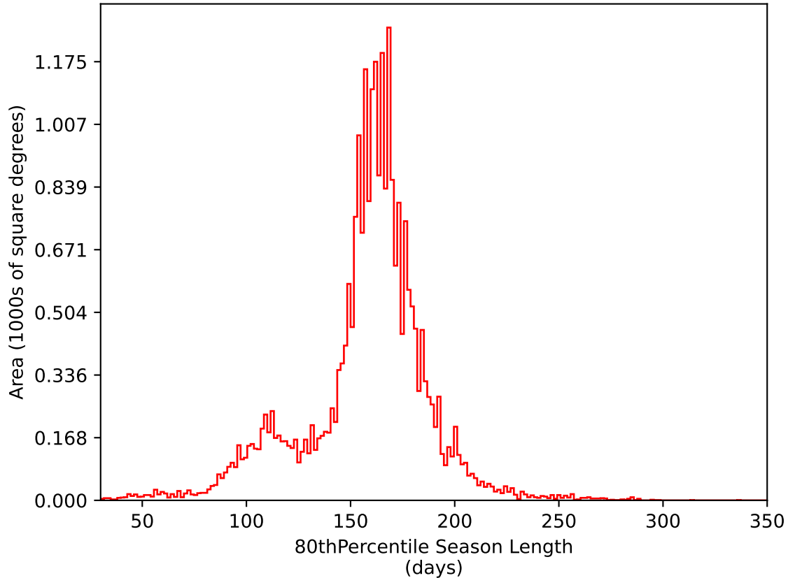
ddf_acor_sf10_lsf40_lsr20_v3.4_10yrs All sky i band: 80thPercentile Season Length
