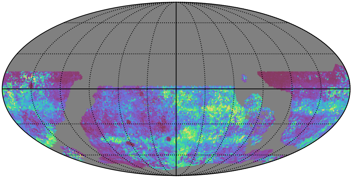
ddf_acor_sf10_lsf40_lsr20_v3.4_10yrs WFD zy bands: 75th Percentile Intranight Timespan
