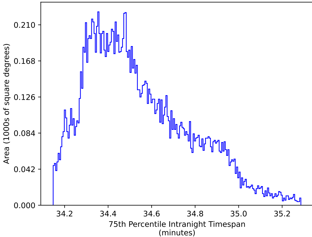
ddf_acor_sf10_lsf40_lsr20_v3.4_10yrs WFD zy bands: 75th Percentile Intranight Timespan
