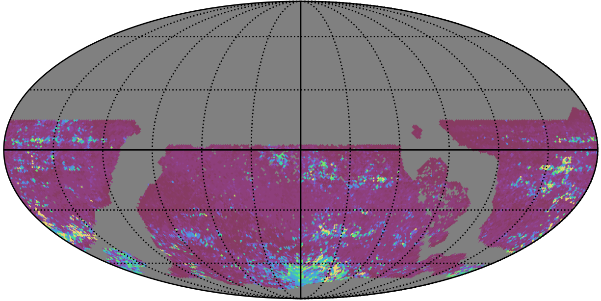
ddf_acor_sf10_lsf40_lsr20_v3.4_10yrs WFD z band: 75th Percentile Intranight Timespan
