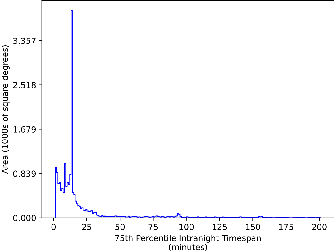
ddf_acor_sf10_lsf40_lsr20_v3.4_10yrs WFD z band: 75th Percentile Intranight Timespan
