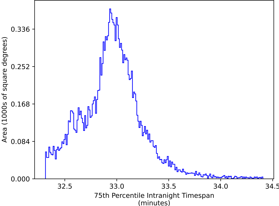
ddf_acor_sf10_lsf40_lsr20_v3.4_10yrs WFD y band: 75th Percentile Intranight Timespan
