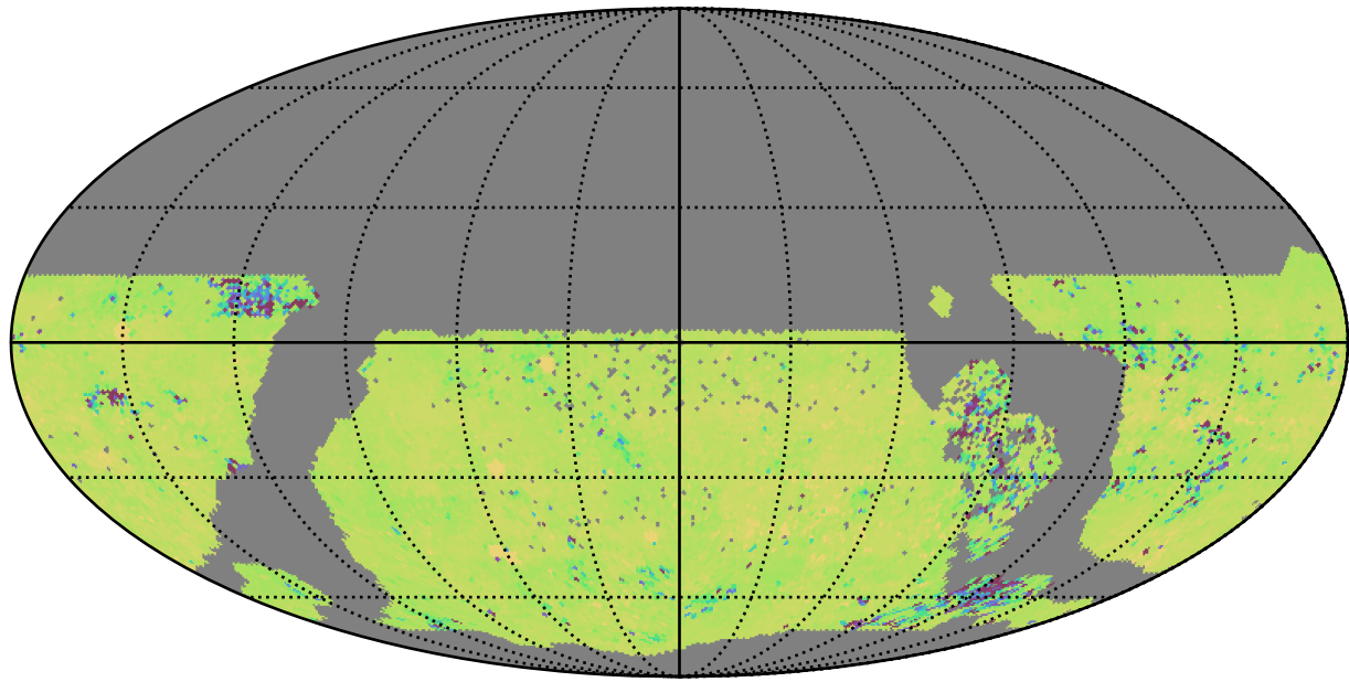
ddf_acor_sf10_lsf40_lsr20_v3.4_10yrs WFD ug bands: 75th Percentile Intranight Timespan
