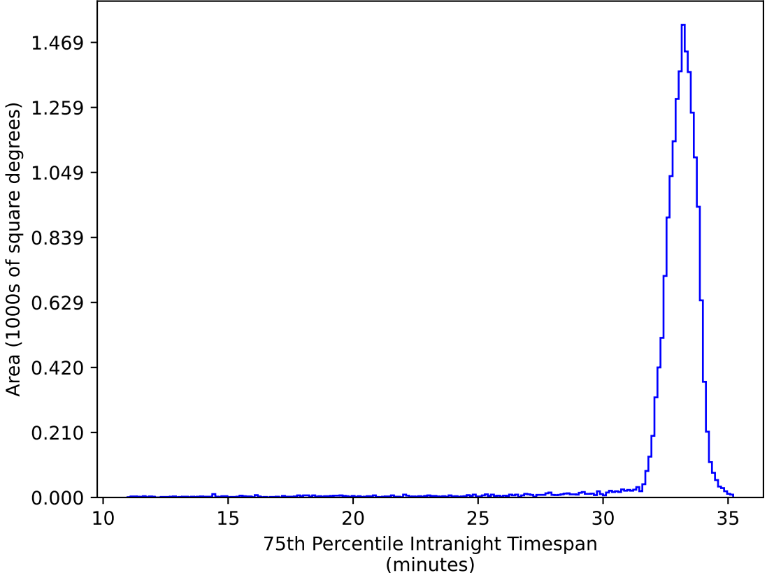
ddf_acor_sf10_lsf40_lsr20_v3.4_10yrs WFD ug bands: 75th Percentile Intranight Timespan
