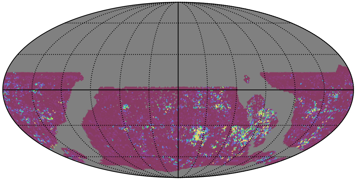
ddf_acor_sf10_lsf40_lsr20_v3.4_10yrs WFD u band: 75th Percentile Intranight Timespan
