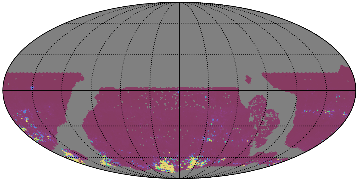
ddf_acor_sf10_lsf40_lsr20_v3.4_10yrs WFD ri bands: 75th Percentile Intranight Timespan
