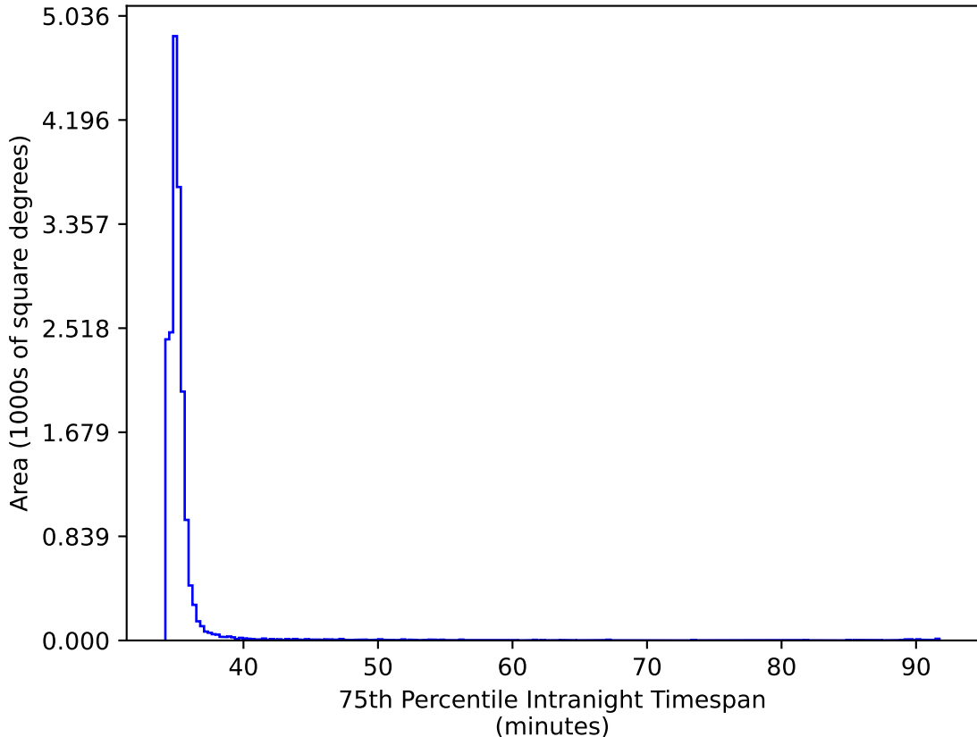
ddf_acor_sf10_lsf40_lsr20_v3.4_10yrs WFD ri bands: 75th Percentile Intranight Timespan
