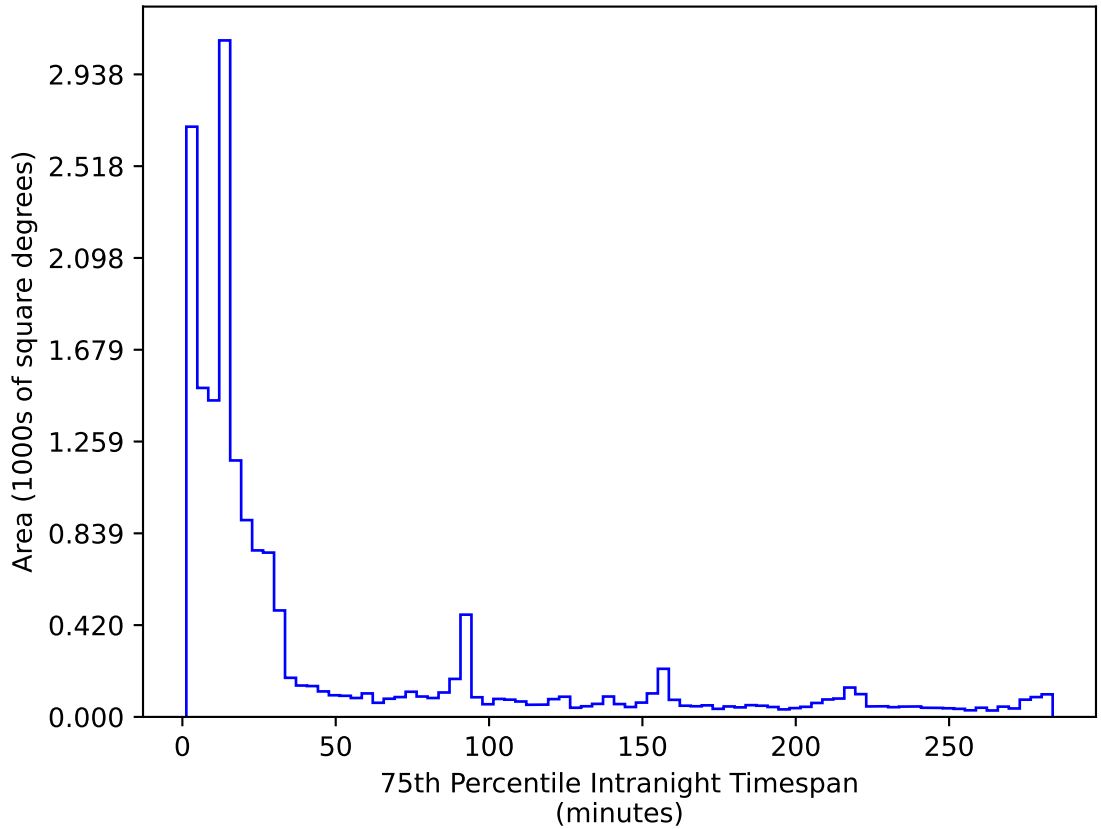
ddf_acor_sf10_ls40_lsr20_v3.4_10yrs WFD r band: 75th Percentile Intranight Timespan
