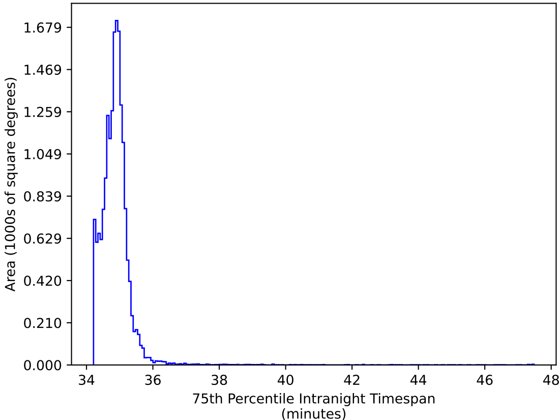
ddf_acor_sf10_lsf40_lsr20_v3.4_10yrs WFD iz bands: 75th Percentile Intranight Timespan
