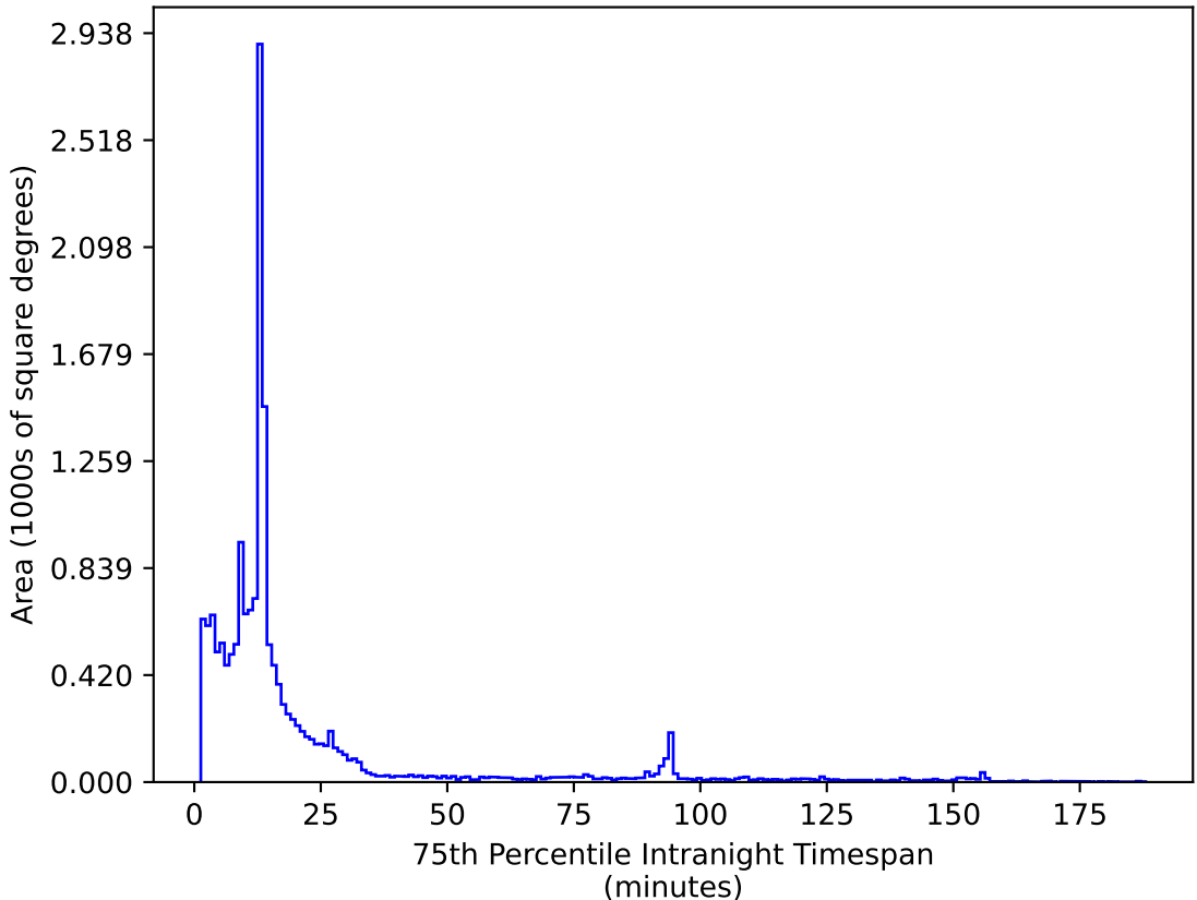
ddf_acor_sf10_ls40_lsr20_v3.4_10yrs WFD i band: 75th Percentile Intranight Timespan
