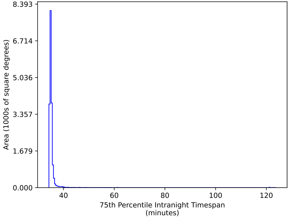
ddf_acor_sf10_lsf40_lsr20_v3.4_10yrs WFD gr bands: 75th Percentile Intranight Timespan
