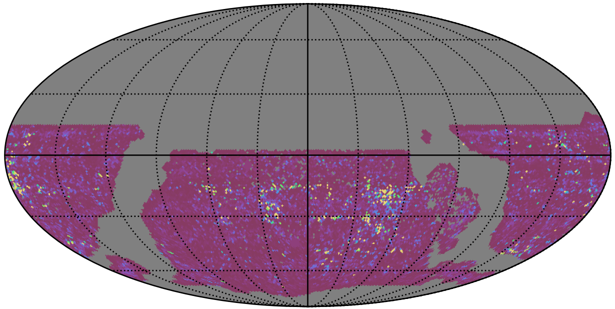
ddf_acor_sf10_lsf40_lsr20_v3.4_10yrs WFD g band: 75th Percentile Intranight Timespan
