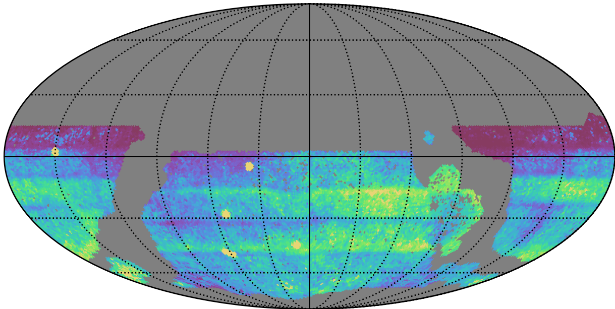
ddf_acor_sf10_lsf40_lsr20_v3.4_10yrs WFD all bands: 75th Percentile Intranight Timespan
