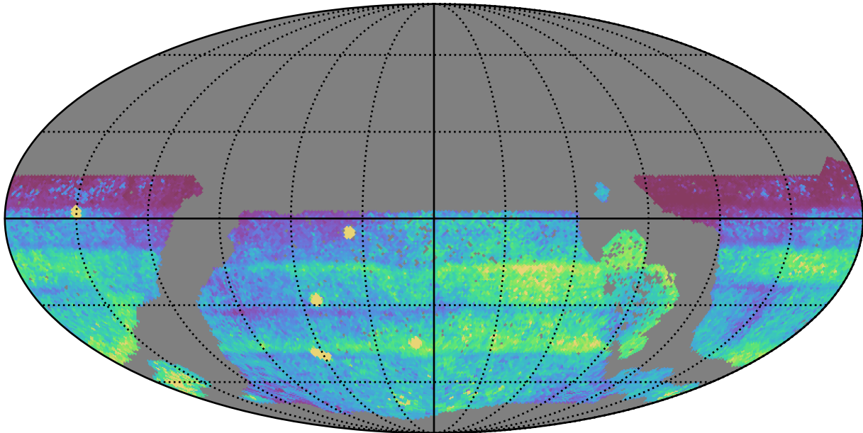
ddf_acor_sf10_lsf40_lsr20_v3.4_10yrs WFD: 75th Percentile Intranight Timespan
