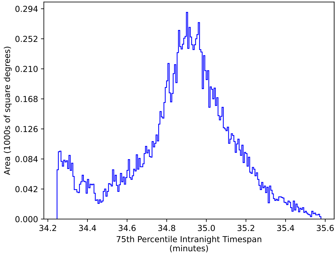
ddf_acor_sf10_lsf40_lsr20_v3.4_10yrs WFD: 75th Percentile Intranight Timespan
