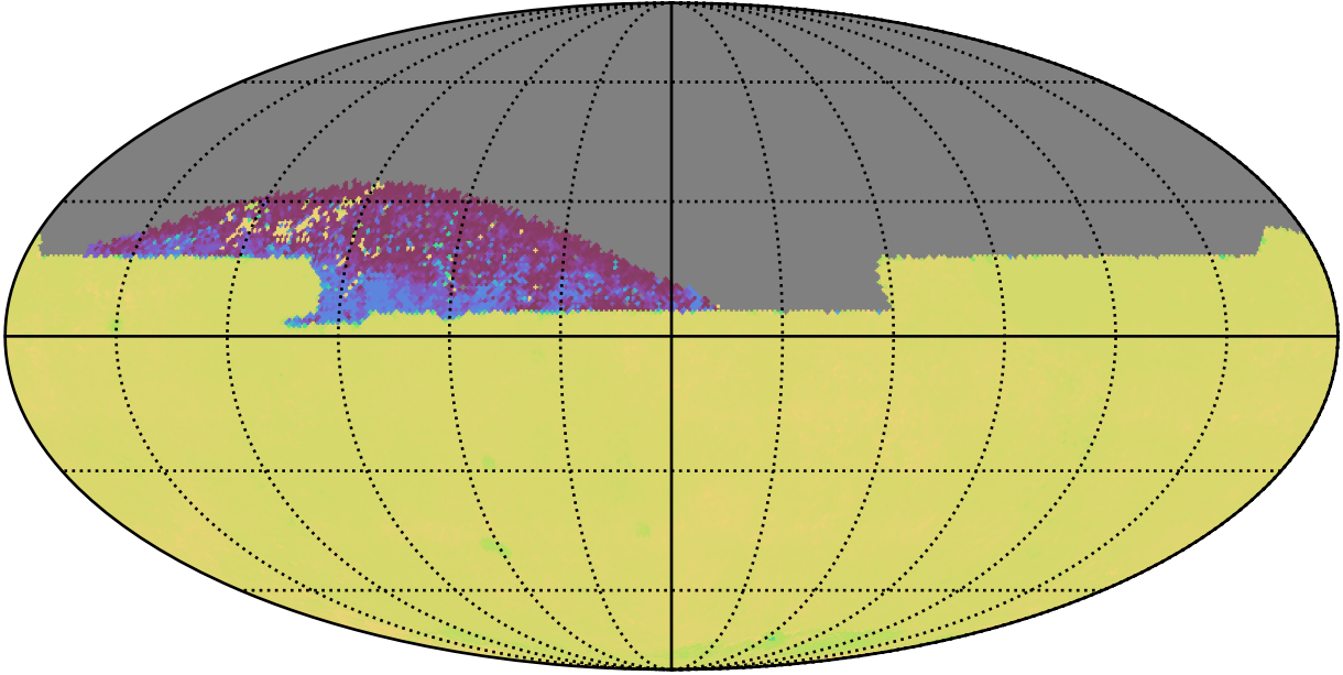
ddf_acor_sf10_lsf40_lsr20_v3.4_10yrs All sky zy bands: 75th Percentile Intranight Timespan
