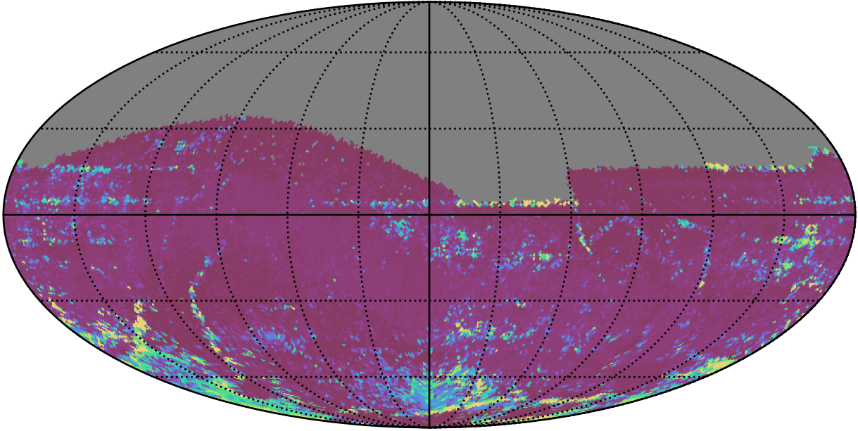
ddf_acor_sf10_lsf40_lsr20_v3.4_10yrs All sky z band: 75th Percentile Intranight Timespan
