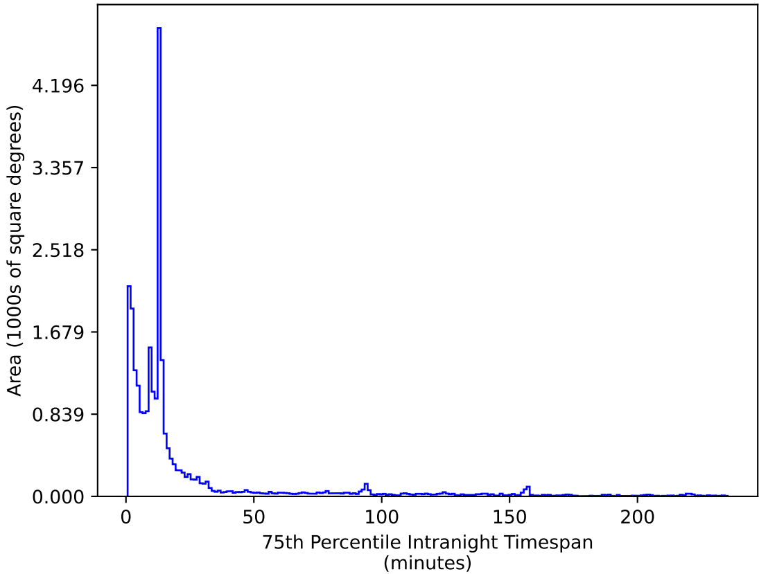
ddf_acor_sf10_lsf40_lsr20_v3.4_10yrs All sky z band: 75th Percentile Intranight Timespan
