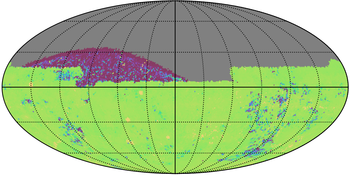
ddf_acor_sf10_lsf40_lsr20_v3.4_10yrs All sky ug bands: 75th Percentile Intranight Timespan
