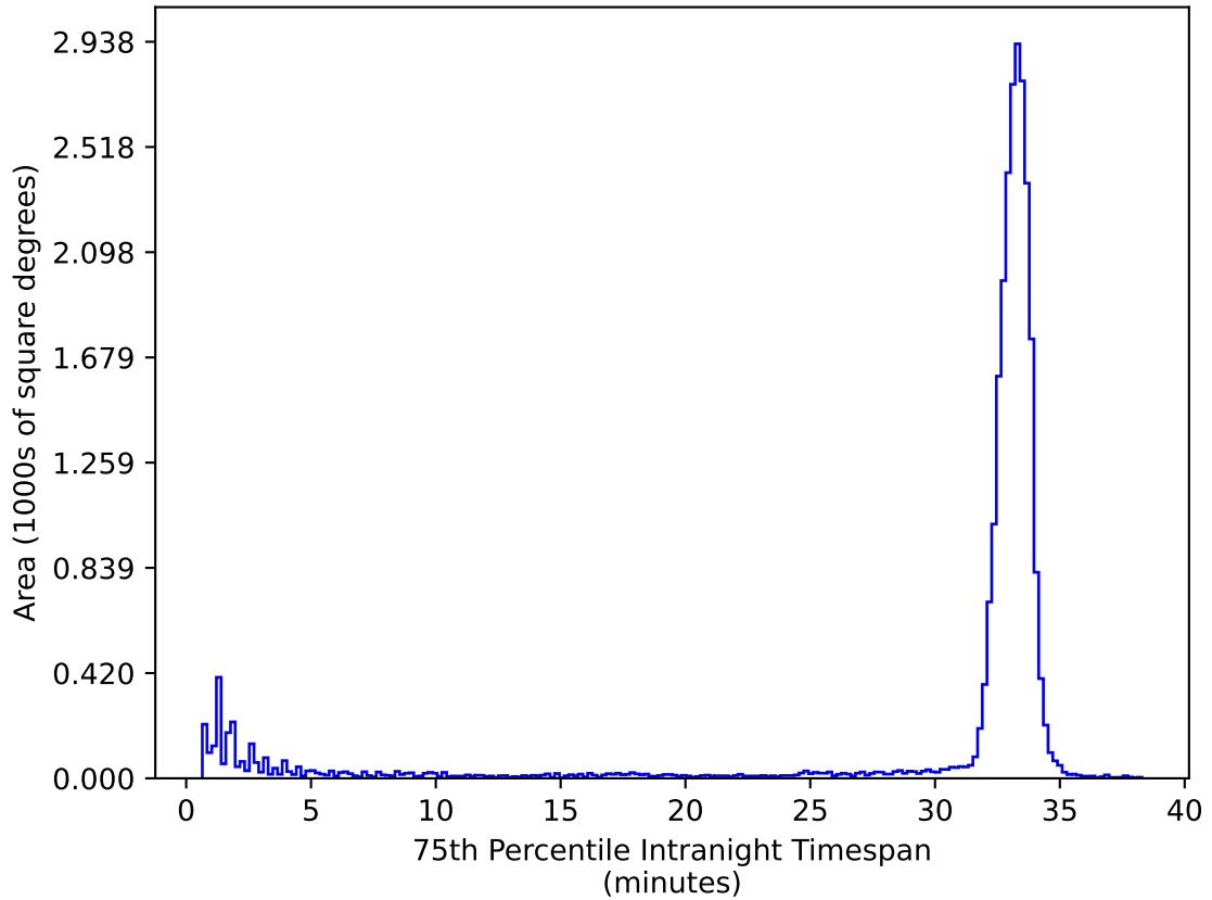
ddf_acor_sf10_lsf40_lsr20_v3.4_10yrs All sky ug bands: 75th Percentile Intranight Timespan
