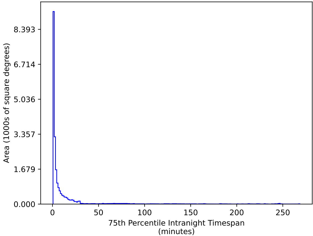
ddf_acor_sf10_lsf40_lsr20_v3.4_10yrs All sky u band: 75th Percentile Intranight Timespan
